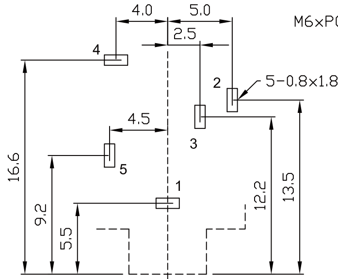
P.C.B. LAYOUT(±0.1) (BOTTOM VIEW)
