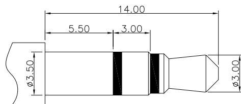
ø3.50mm 3 POLE PLUG
