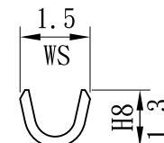
B-B Section
