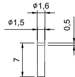
Female pin
