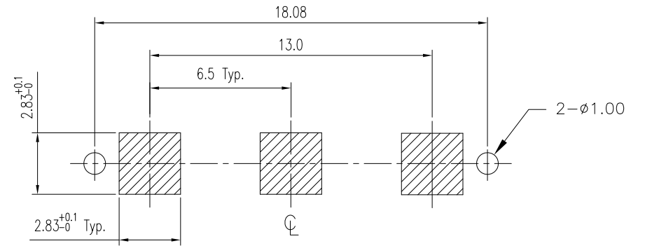
Recommended P.C.B. Layout Layout Tolerance = ± 0.05 mm
