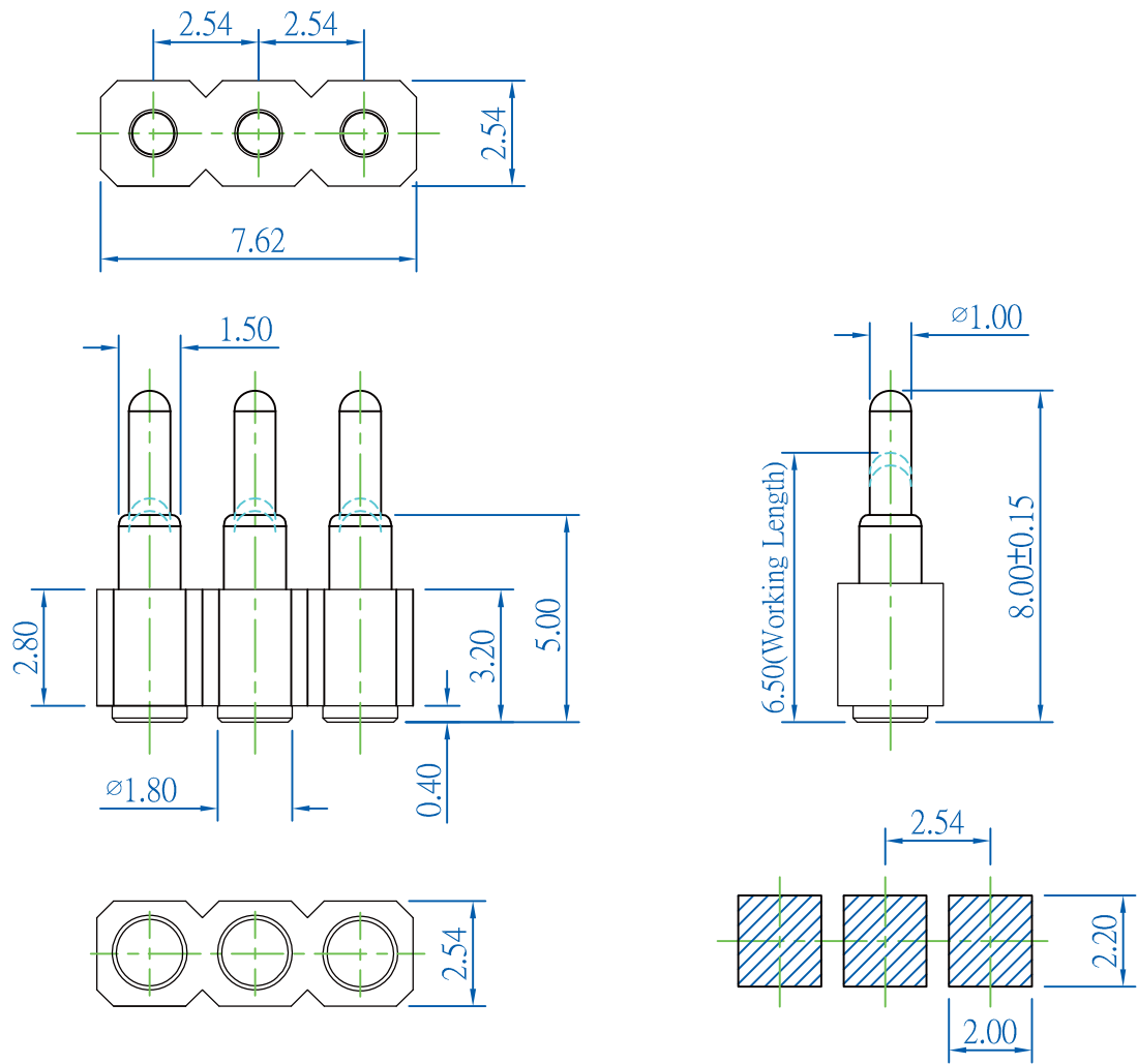
RECOMMENDE PCB LAYOUT
