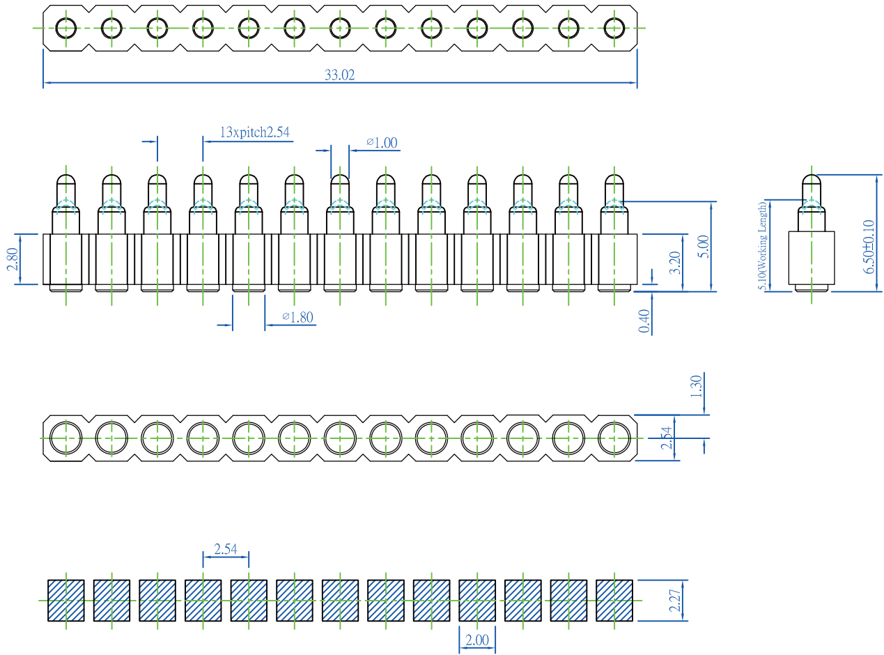
RECOMMENDE PCB LAYOUT
