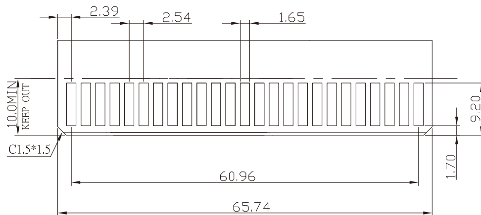
RECOMMENDED MATTING BOARD FOOTPRINT (Tolerance:±0.05)
