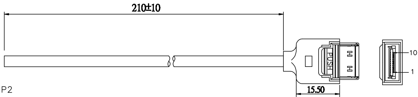
P1 PCMCIA-10PIN
