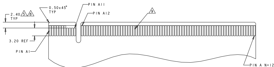
ExpressModule LAYOUT (MATING PART ONLY)
