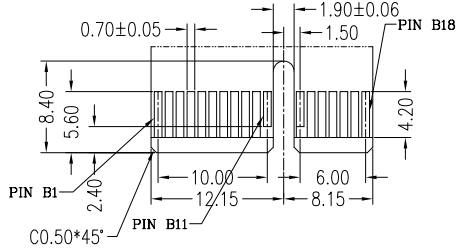
Primary (Component) Side
