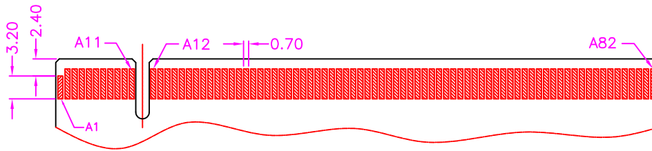
ADD-IN CARD EDGE-FINGER DIMENSIONS
