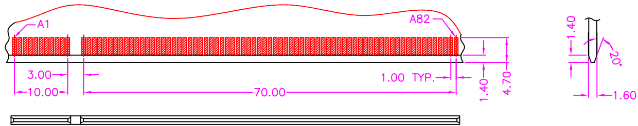
ADD-IN CARD EDGE-FINGER DIMENSIONS
