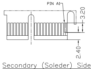
Secondary (Solder) Side
