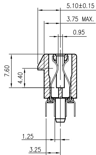
SECTION F-F
