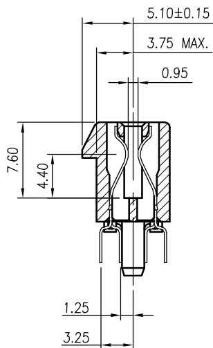
SECTION F-F
