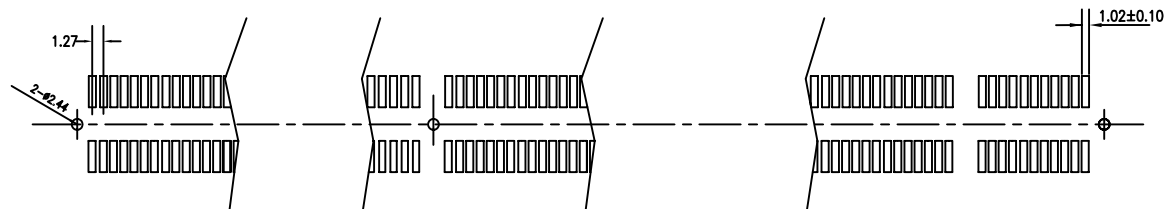
RECOMMENDED PCB LAYOUT (TOP VIEW)
