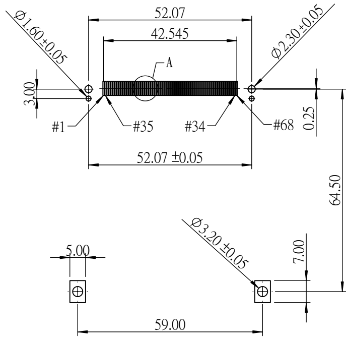
PCB LAYOUT : COMPONENT SIDE
