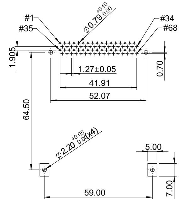
PCB LAYOUT : COMPONENT SIDE PCB THK. 1.60±0.10
