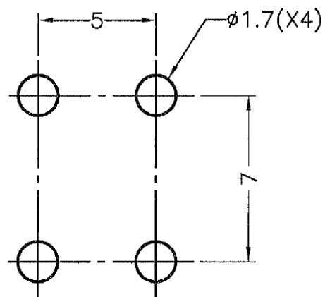
MOUNTING HOLE
