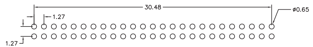
Recommended P.C.B Layout
