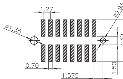
Recommended P.C.Board Layout (Tolerance: \pm 0.05 )
