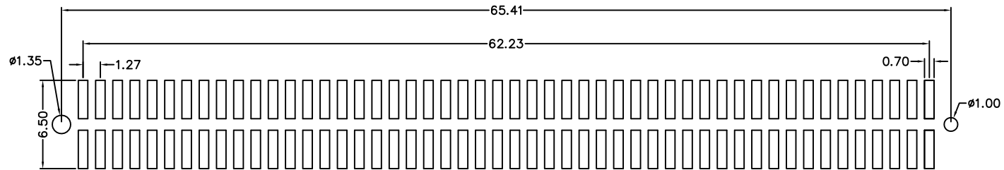
Recommended P.C.B Layout
