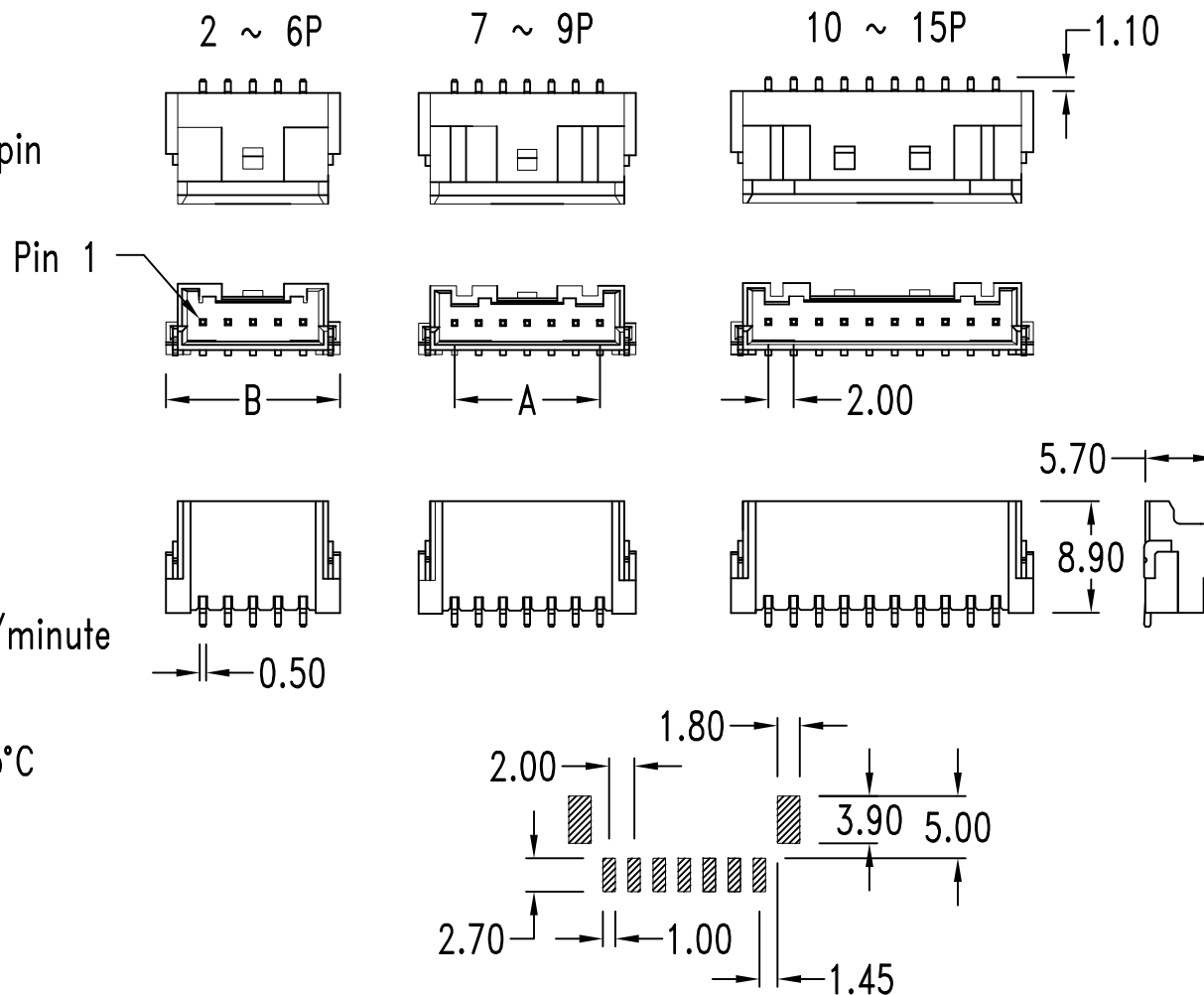
P. C. board hole dimensions
