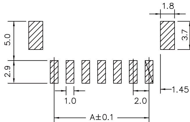
RECOMMENDED P.C.BOARD LAYOUT DIMM.
