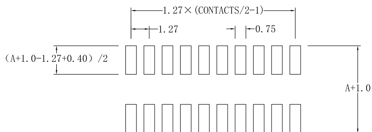
P. C. B . LAYOUT
