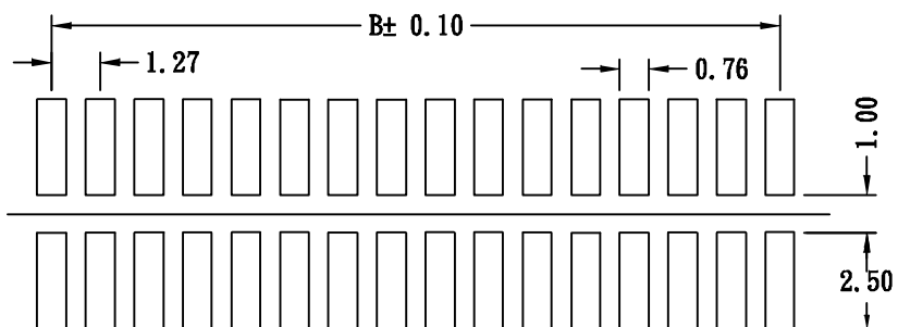
P. C. B LAYOUT (TOL. : ± 0.05)
