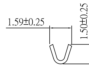
B-B SECTION
