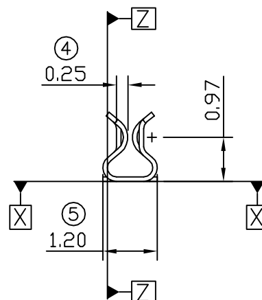
PCB Recommend Layout Pattern
