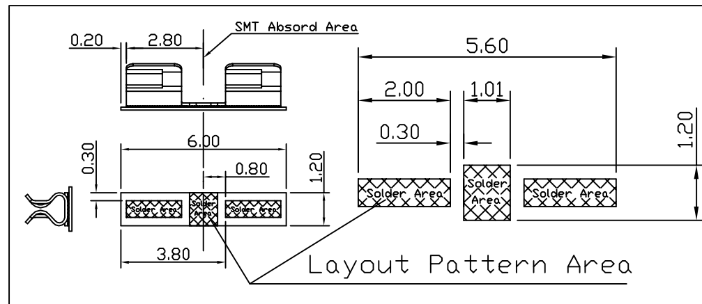
PCB Recommend Layout Pattern
