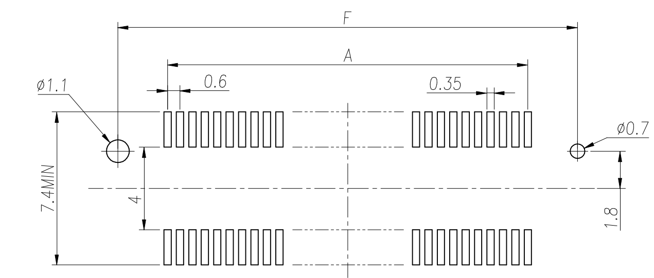
RECOMMENDED PCB LAYOUT (TOP VIEW) (DIMENSION SHOWN IS FOR CONNECTOR WITH POSTS)
