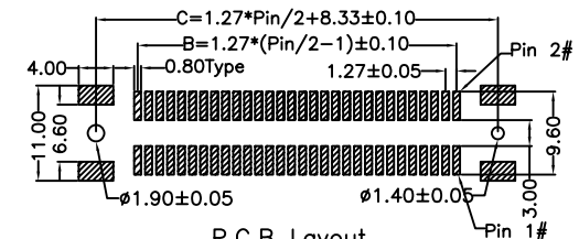
P.C.B Layout (Component Side View)
