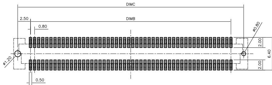
RECOMMEND PCB LAYOUT TOLERANCE±0.05mm
