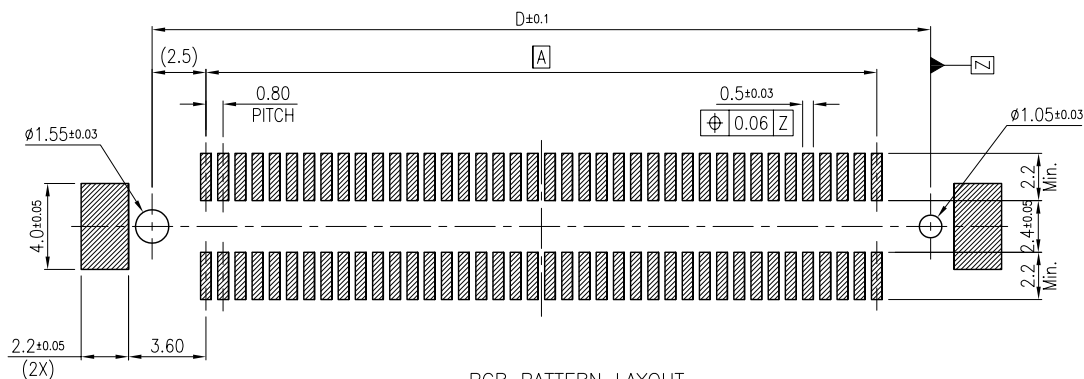
PCB PATTERN LAYOUT
