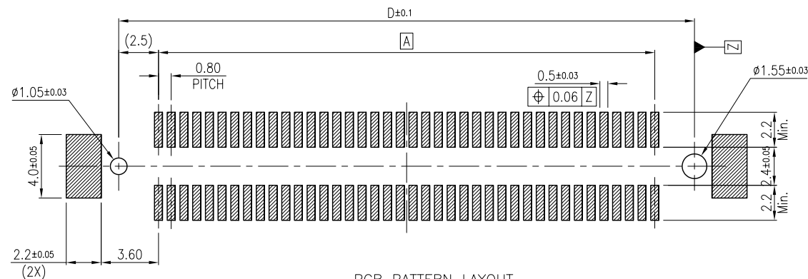
PCB PATTERN LAYOUT
