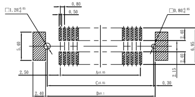
PCB PATTERN LAYOUT
