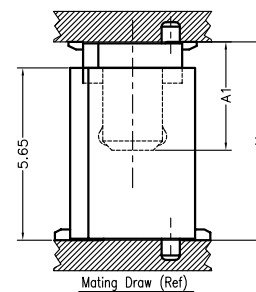
**Mating Height Dimension
