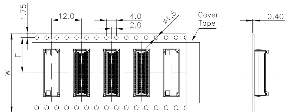
For Reel width (dimension W)32,44,56,72mm Double rows hole
