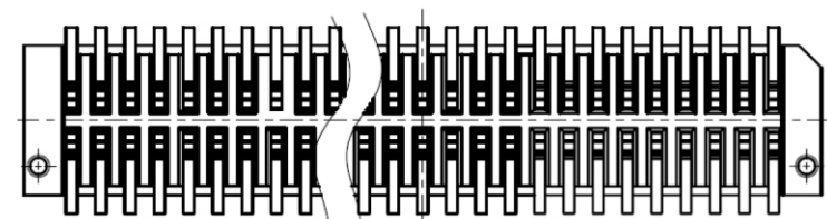
Contacts Dimensions
