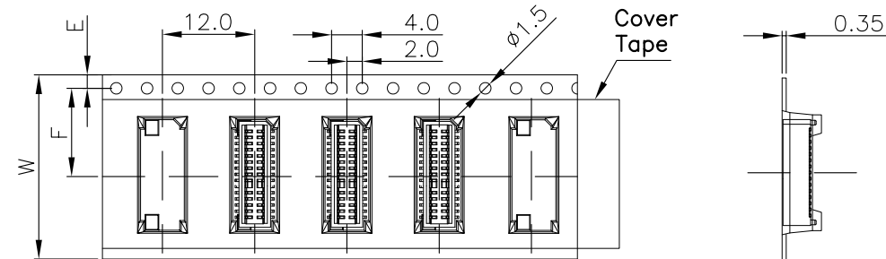
For Reel width (dimension W)16,24mm Single row hole
