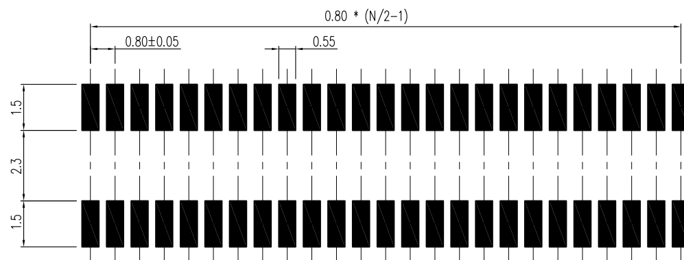
PCB Layout For Surface Mounting
