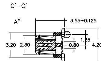
0.80mm(.031")Pitch Board-to-Board Plug
