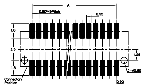
PCB Layout For Surface Mounting
