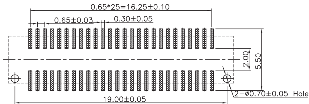
PCB LAYOUT
