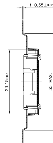
C-C SECTION
