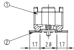
DETAIL FOR SOLDERING AREA
