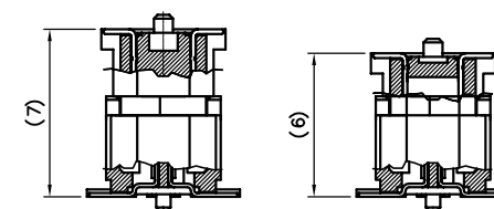
MATED CONDITION (REF.)
