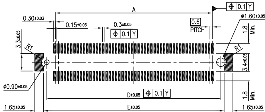
PCB PATTERN LAYOUT
