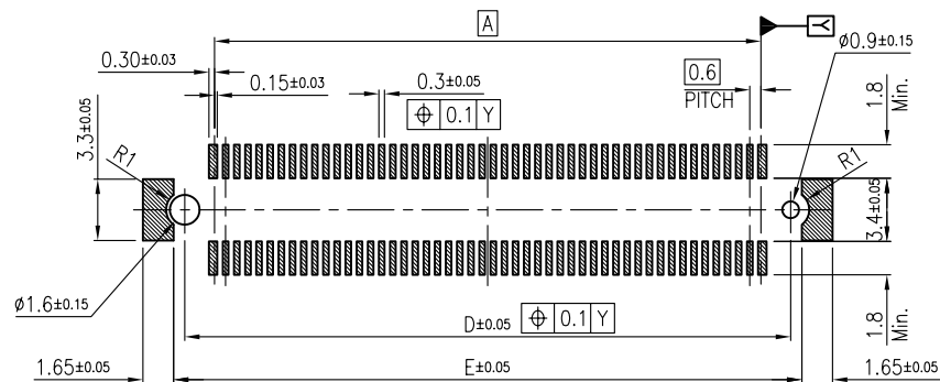
PCB PATTERN LAYOUT
