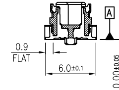
SEC. Z-Z (GROUND POSITION)
