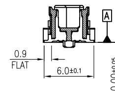
SEC. Y-Y (SIGNAL POSITION)
