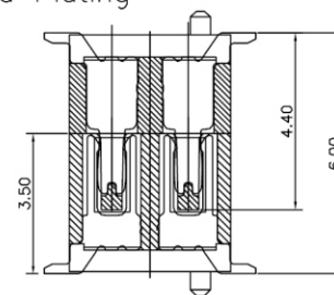
Mating Draw (Ref)
