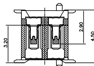
Mating Drawing (Ref)
