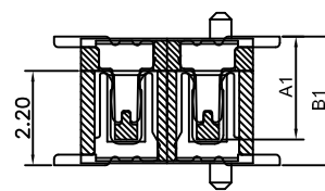
Mating Drawing (Ref)
