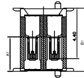
Mating Draw (Ref)
