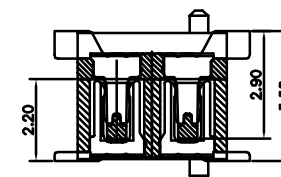
Mating Draw (Ref)
